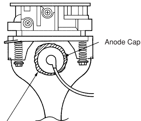
Silicon (On shaded area) TSE3843W #23960136
