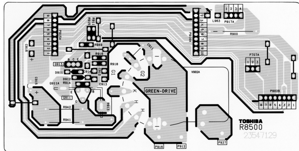
CRD-D G BOARD PD0820A-2 BOTTOM (FOIL) SIDE
