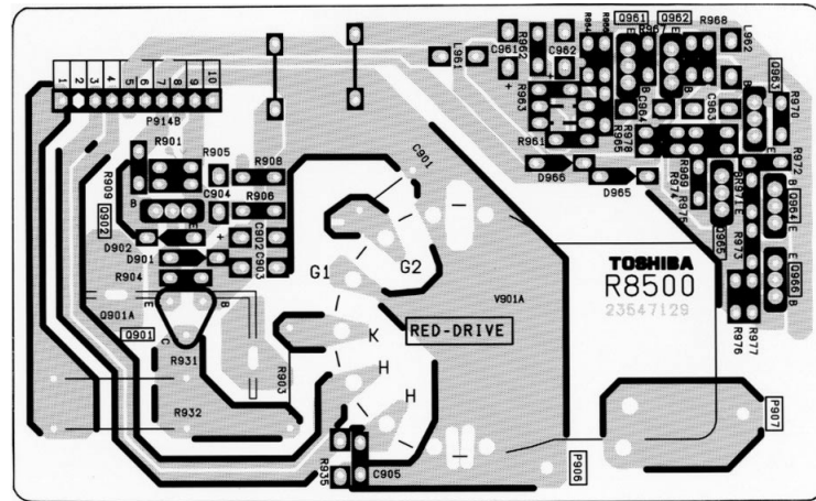
CRD-D R BOARD PD0820A-1 BOTTOM (FOIL) SIDE
