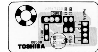
LED BOARD PD0820A-6 BOTTOM (FOIL) SIDE
