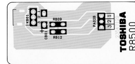
RMT BOARD PD0820A-5 BOTTOM (FOIL) SIDE
