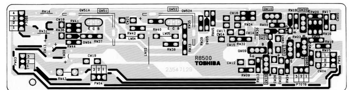
SVM BOARD PD820A-7 BOTTOM (FOIL) SIDE
